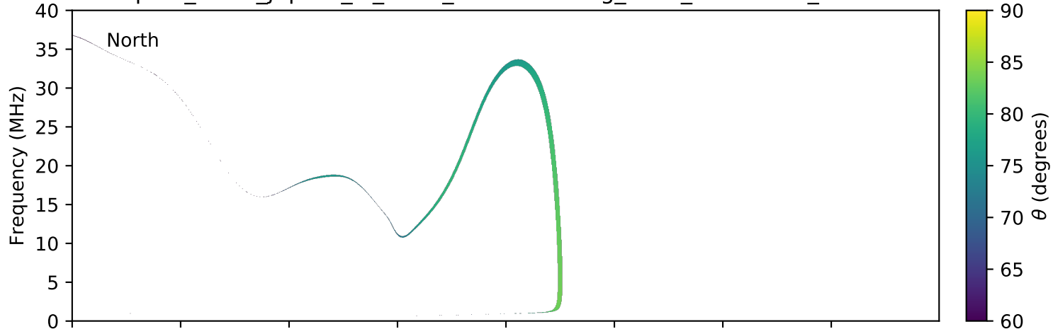
expres_earth_jupiter_io_isaac_lossc-wid1deg_3kev_20080807_v01.cdf
