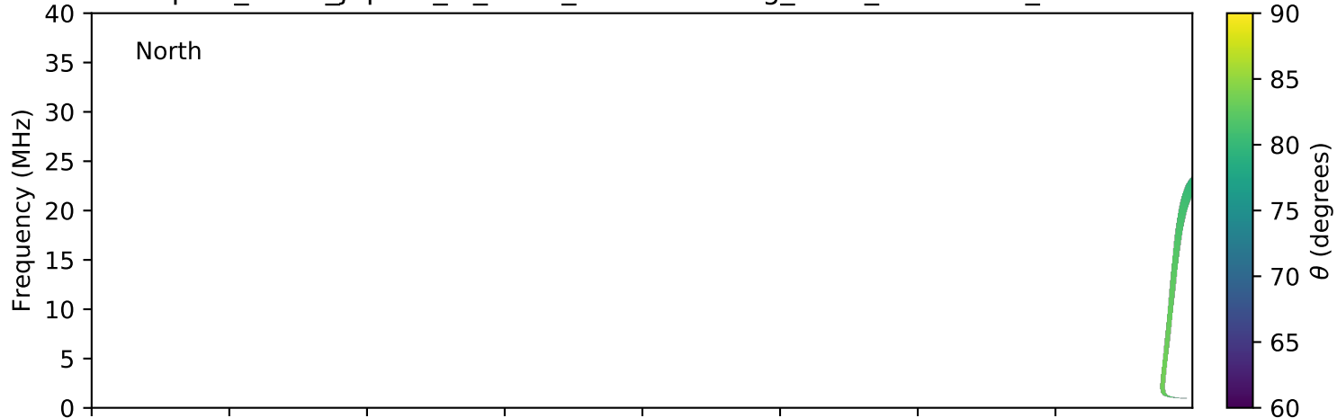
expres_earth_jupiter_io_isaac_lossc-wid1deg_3kev_20080804_v01.cdf
