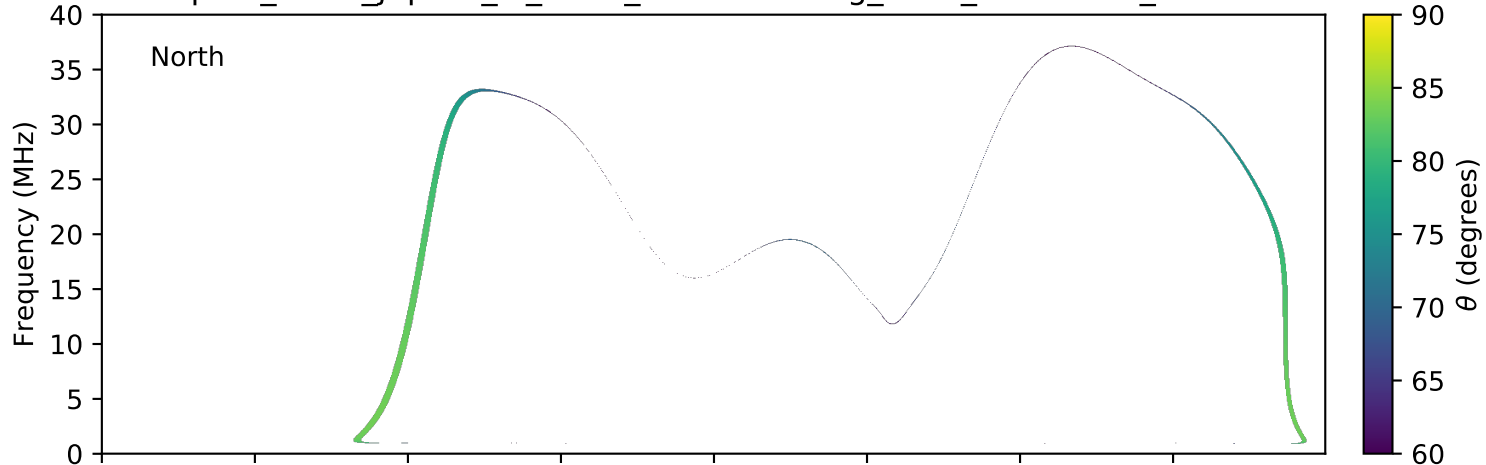
expres_earth_jupiter_io_isaac_lossc-wid1deg_3kev_20080803_v01.cdf
