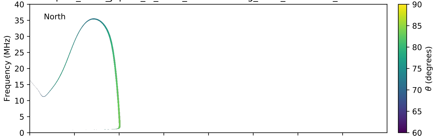
expres_earth_jupiter_io_isaac_lossc-wid1deg_3kev_20080802_v01.cdf
