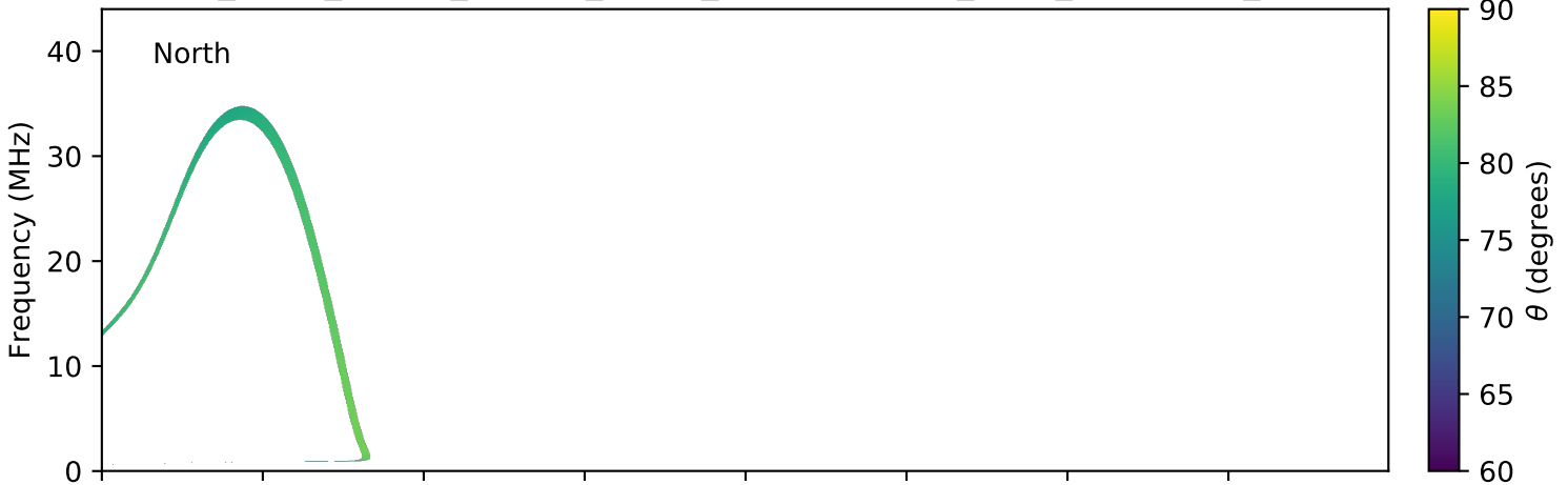
expres_earth_jupiter_europa_jrm09_lossc-wid1deg_3kev_20080823_v01.cdf
