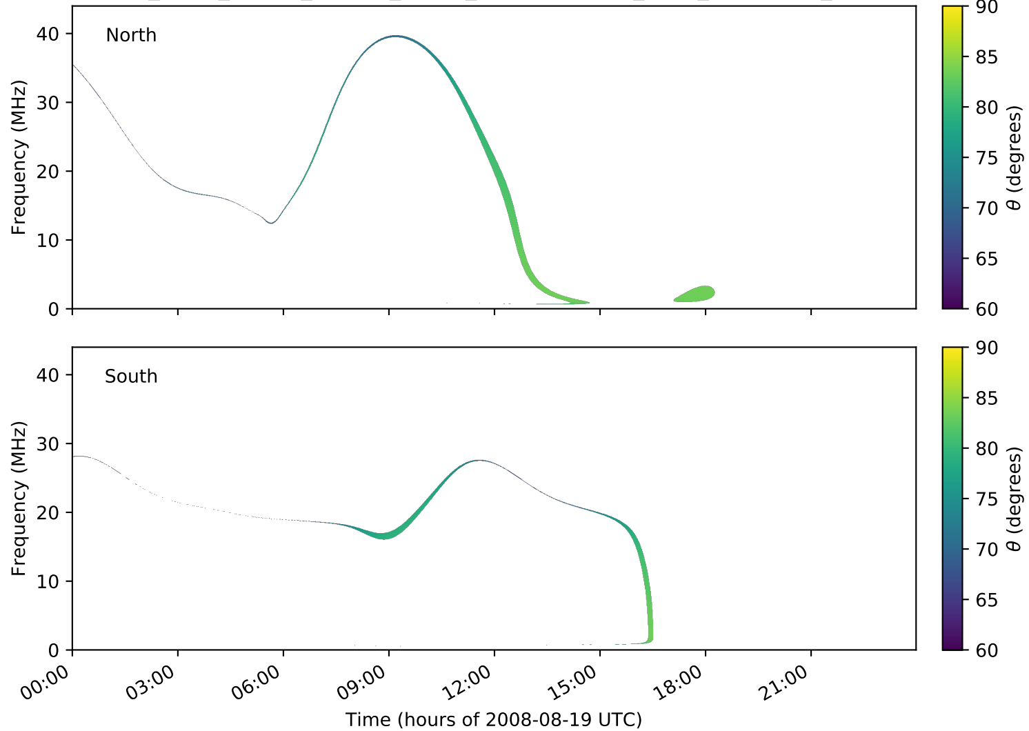
expres_earth_jupiter_europa_jrm09_lossc-wid1deg_3kev_20080819_v01.cdf
