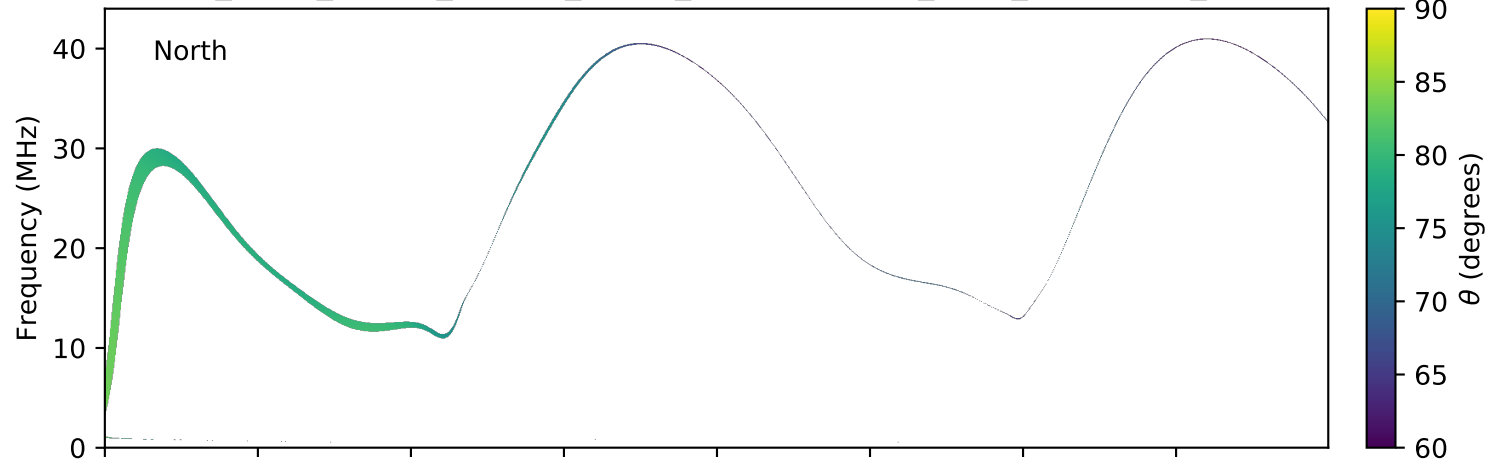
expres_earth_jupiter_europa_jrm09_lossc-wid1deg_3kev_20080811_v01.cdf
