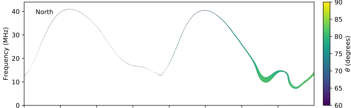
expres_earth_jupiter_europa_jrm09_lossc-wid1deg_3kev_20080808_v01.cdf
