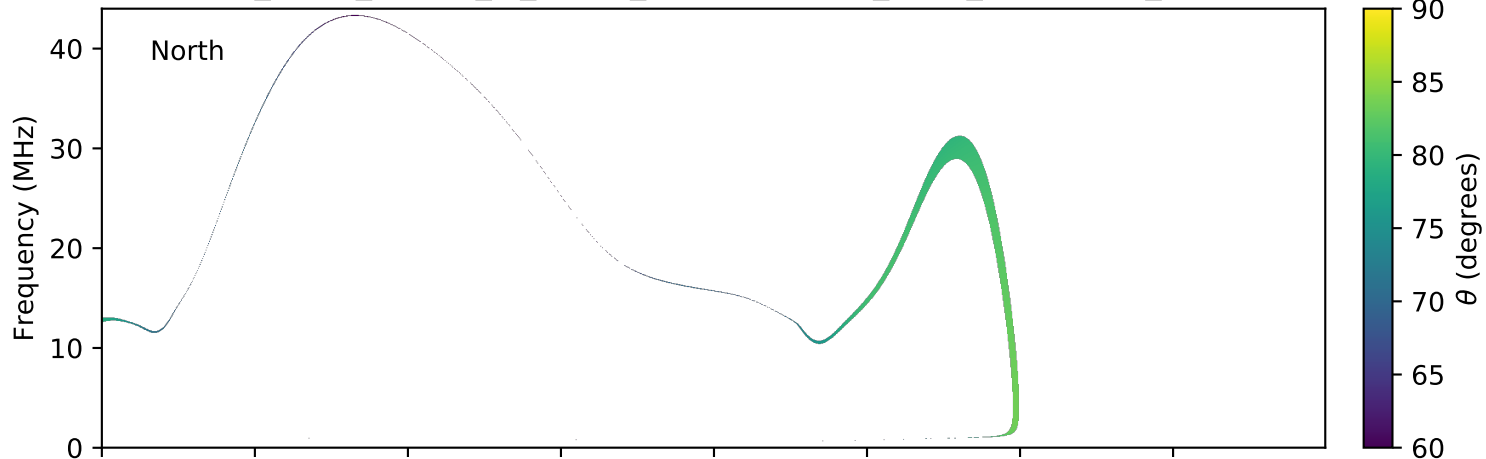
expres_earth_jupiter_io_jrm09_lossc-wid1deg_3kev_20080729_v01.cdf
