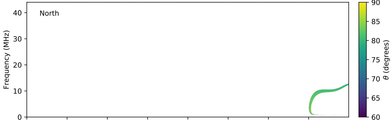
expres_earth_jupiter_io_jrm09_lossc-wid1deg_3kev_20080728_v01.cdf
