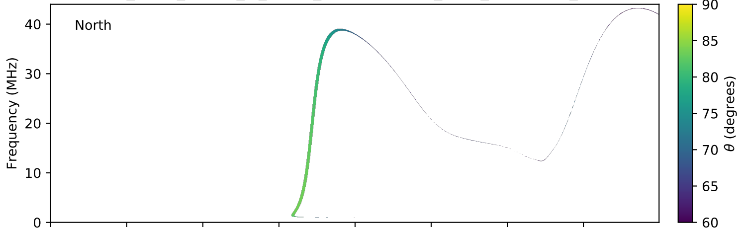
expres_earth_jupiter_io_jrm09_lossc-wid1deg_3kev_20080725_v01.cdf
