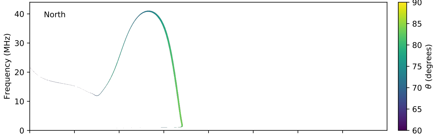
expres_earth_jupiter_io_jrm09_lossc-wid1deg_3kev_20080724_v01.cdf
