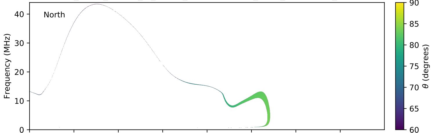
expres_earth_jupiter_io_jrm09_lossc-wid1deg_3kev_20080722_v01.cdf
