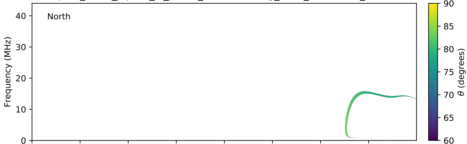
expres_earth_jupiter_io_jrm09_lossc-wid1deg_3kev_20080721_v01.cdf
