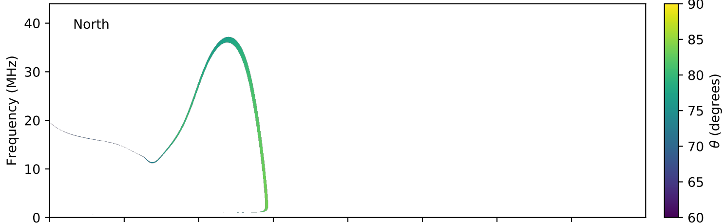
expres_earth_jupiter_io_jrm09_lossc-wid1deg_3kev_20080717_v01.cdf
