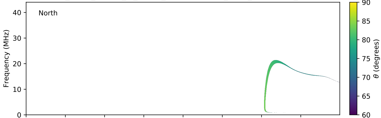
expres_earth_jupiter_io_jrm09_lossc-wid1deg_3kev_20080714_v01.cdf
