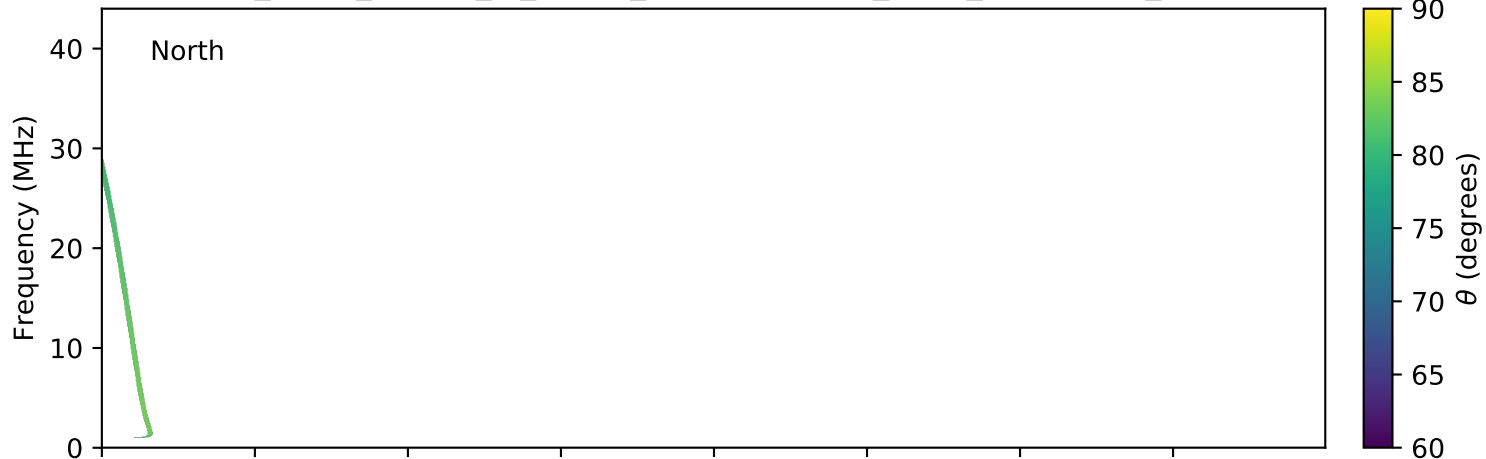
expres_earth_jupiter_io_jrm09_lossc-wid1deg_3kev_20080712_v01.cdf
