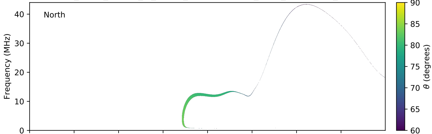
expres_earth_jupiter_io_jrm09_lossc-wid1deg_3kev_20080709_v01.cdf
