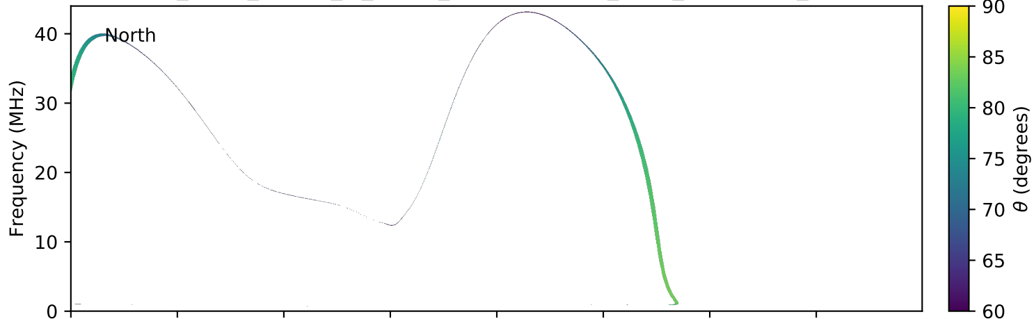
expres_earth_jupiter_io_jrm09_lossc-wid1deg_3kev_20080706_v01.cdf
