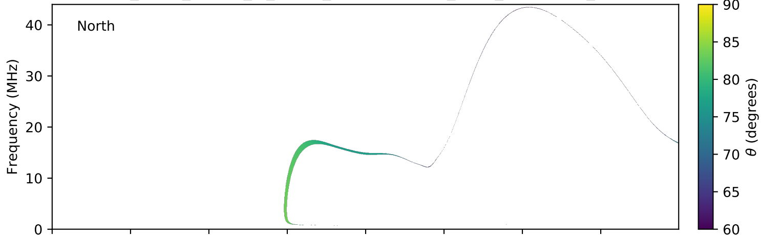
expres_earth_jupiter_io_jrm09_lossc-wid1deg_3kev_20080702_v01.cdf
