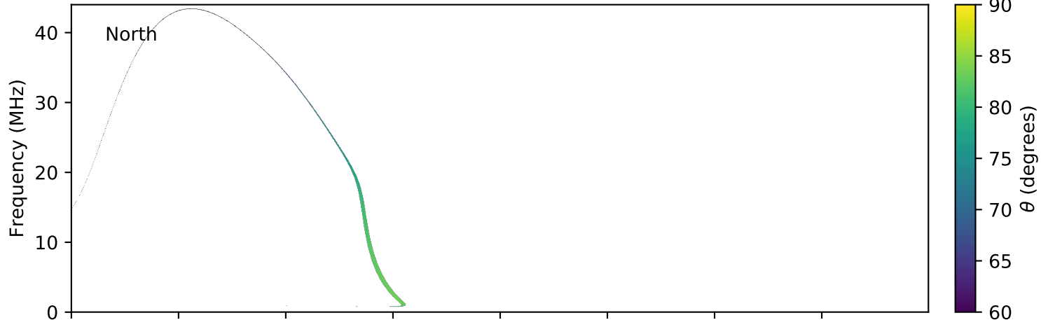
expres_earth_jupiter_io_jrm09_lossc-wid1deg_3kev_20080701_v01.cdf
