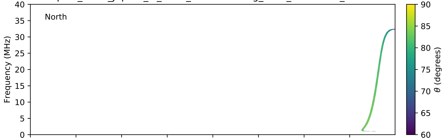
expres_earth_jupiter_io_isaac_lossc-wid1deg_3kev_20080728_v01.cdf
