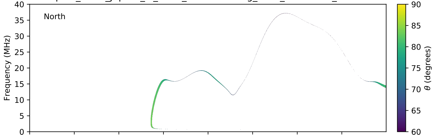
expres_earth_jupiter_io_isaac_lossc-wid1deg_3kev_20080725_v01.cdf
