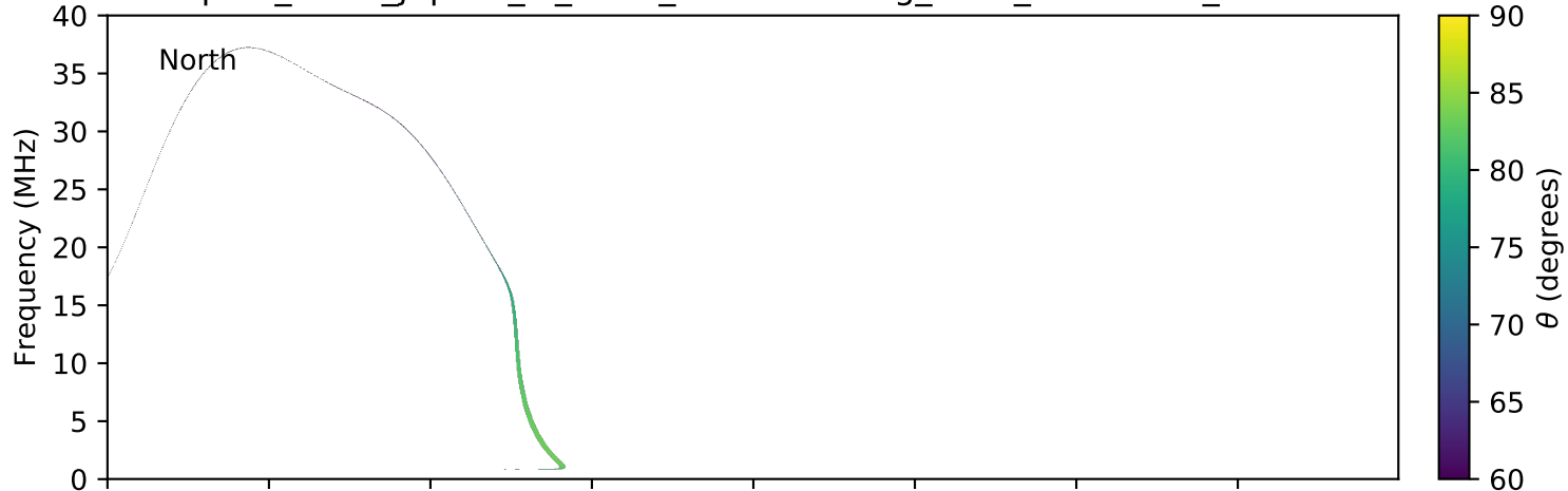
expres_earth_jupiter_io_isaac_lossc-wid1deg_3kev_20080724_v01.cdf
