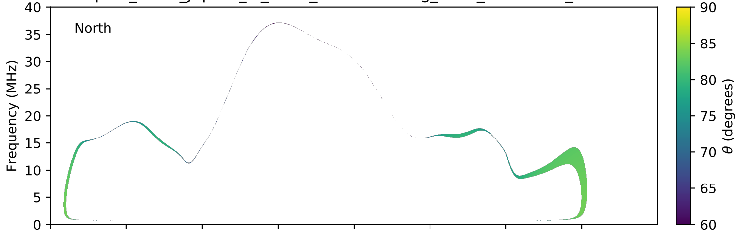
expres_earth_jupiter_io_isaac_lossc-wid1deg_3kev_20080720_v01.cdf
