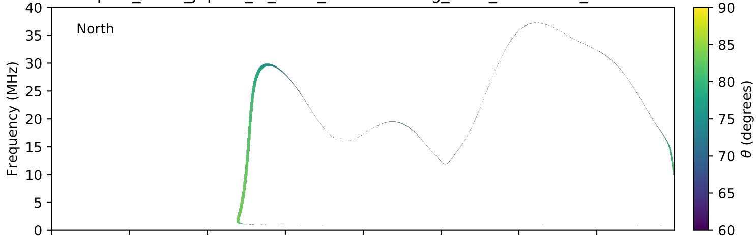
expres_earth_jupiter_io_isaac_lossc-wid1deg_3kev_20080718_v01.cdf
