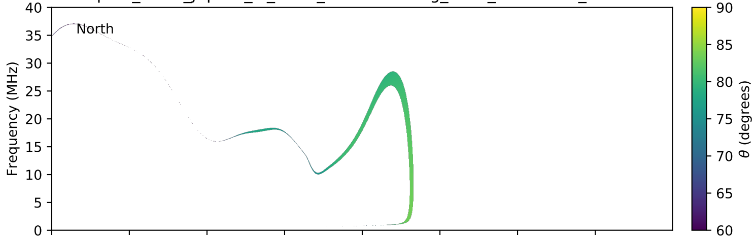
expres_earth_jupiter_io_isaac_lossc-wid1deg_3kev_20080715_v01.cdf
