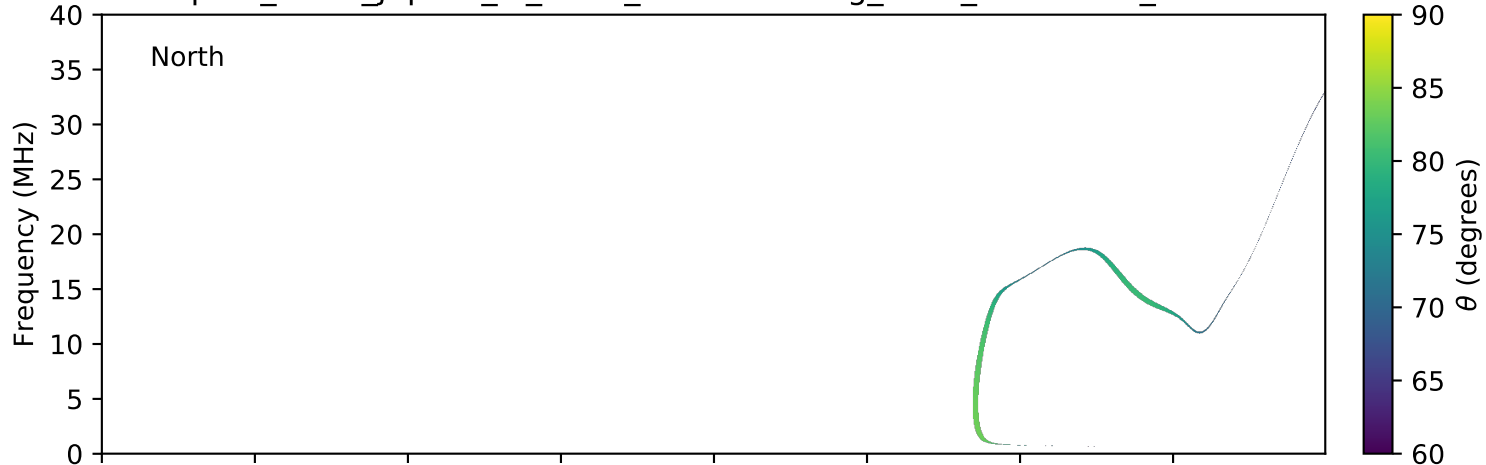
expres_earth_jupiter_io_isaac_lossc-wid1deg_3kev_20080714_v01.cdf
