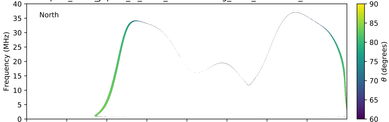
expres_earth_jupiter_io_isaac_lossc-wid1deg_3kev_20080711_v01.cdf
