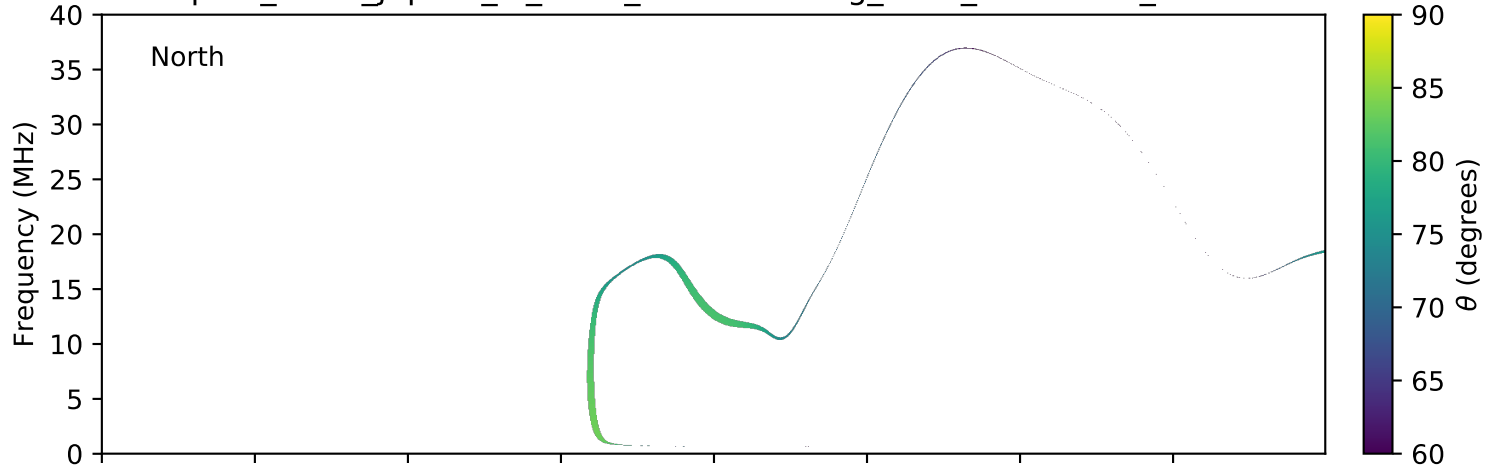
expres_earth_jupiter_io_isaac_lossc-wid1deg_3kev_20080709_v01.cdf
