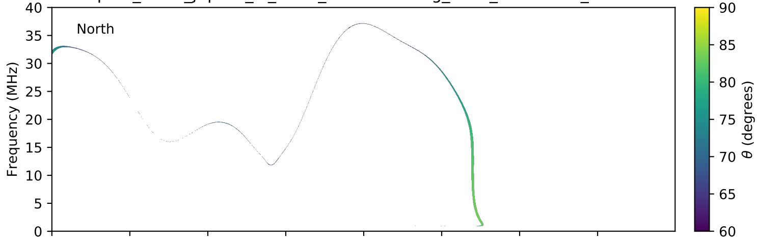
expres_earth_jupiter_io_isaac_lossc-wid1deg_3kev_20080706_v01.cdf
