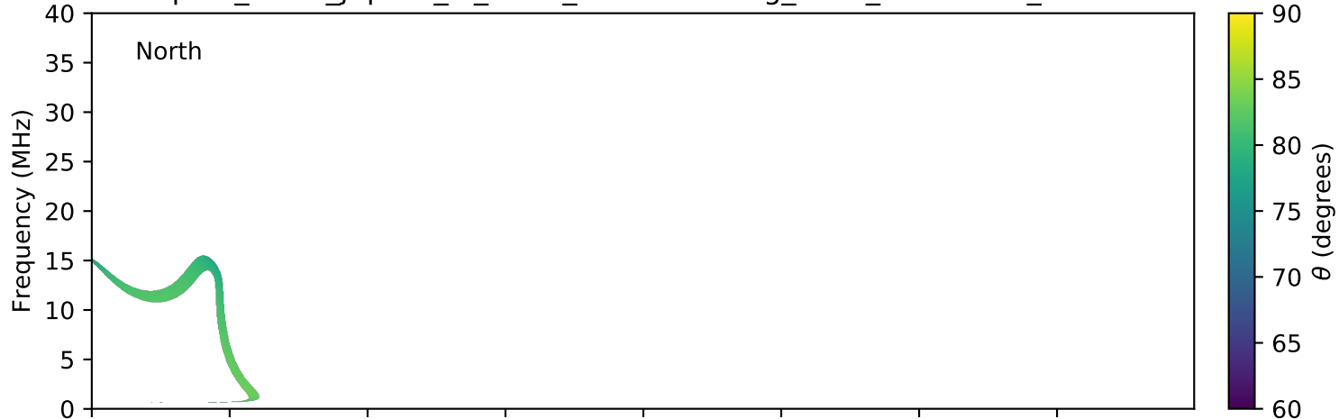
expres_earth_jupiter_io_isaac_lossc-wid1deg_3kev_20080703_v01.cdf
