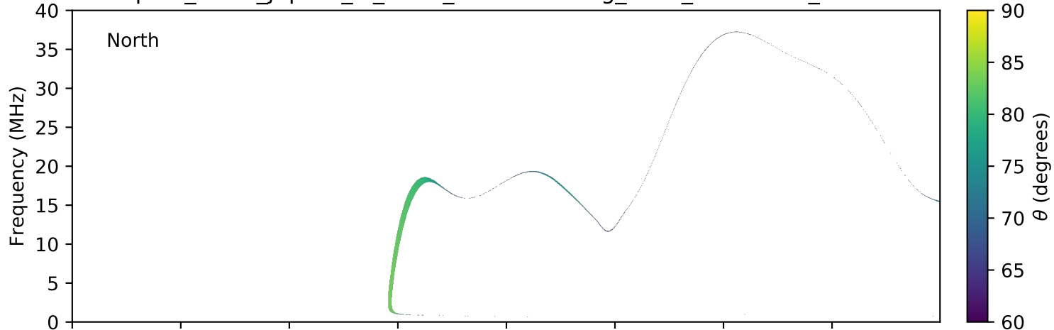
expres_earth_jupiter_io_isaac_lossc-wid1deg_3kev_20080702_v01.cdf
