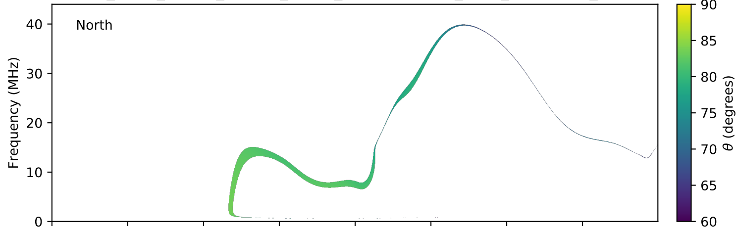
expres_earth_jupiter_europa_jrm09_lossc-wid1deg_3kev_20080731_v01.cdf
