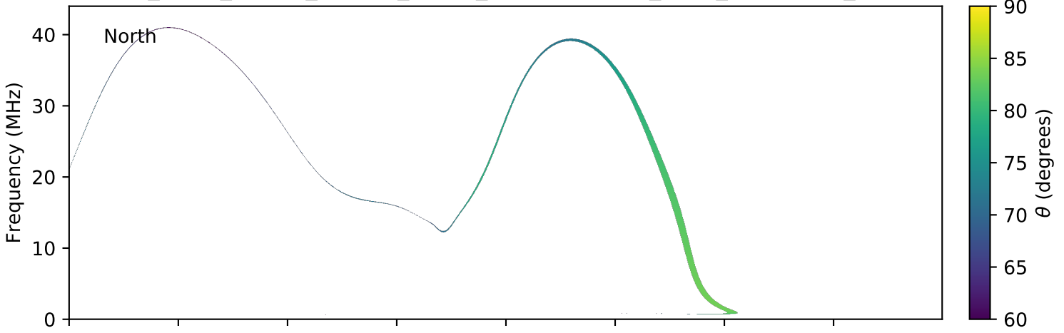
expres_earth_jupiter_europa_jrm09_lossc-wid1deg_3kev_20080725_v01.cdf
