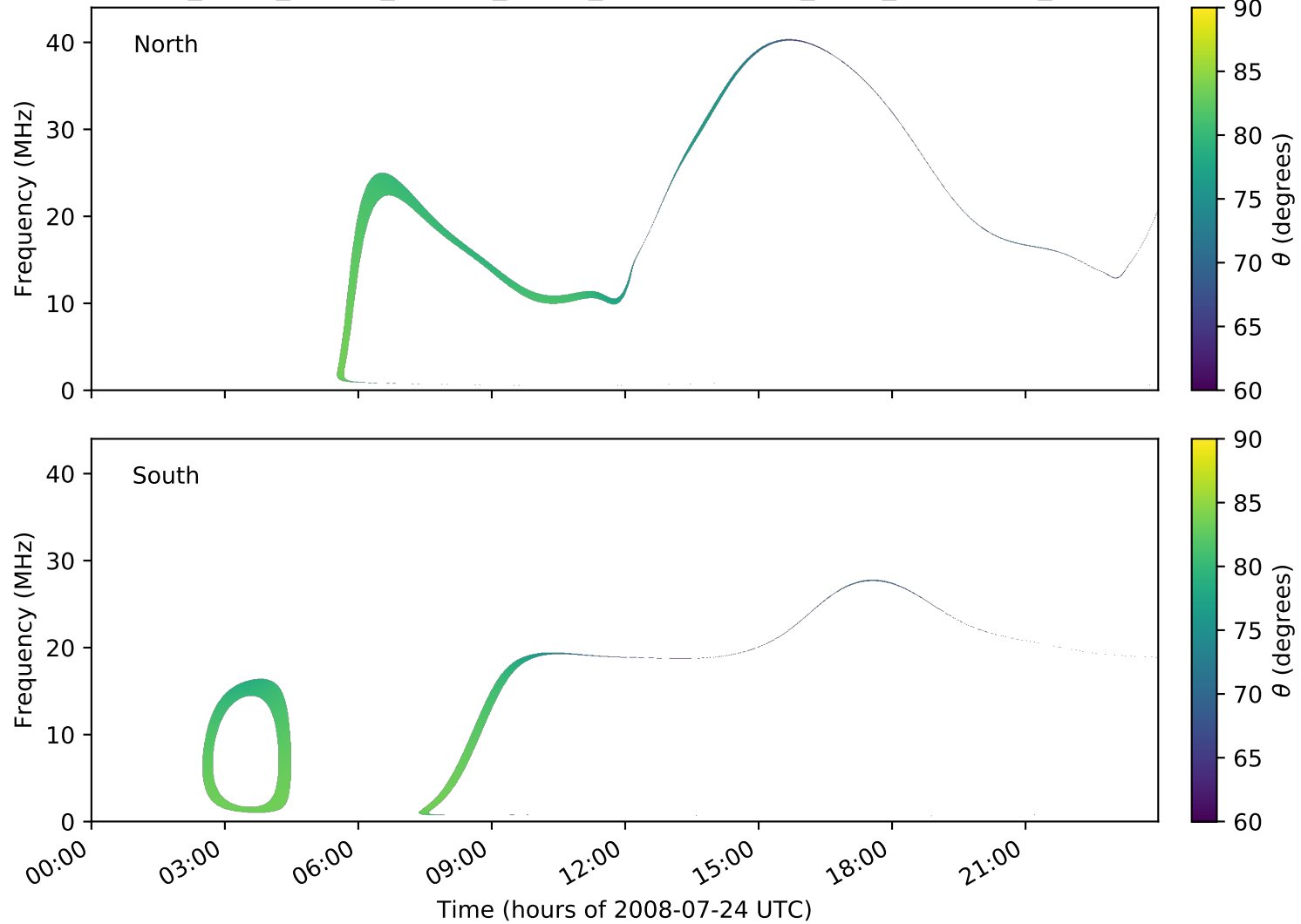
expres_earth_jupiter_europa_jrm09_lossc-wid1deg_3kev_20080724_v01.cdf
