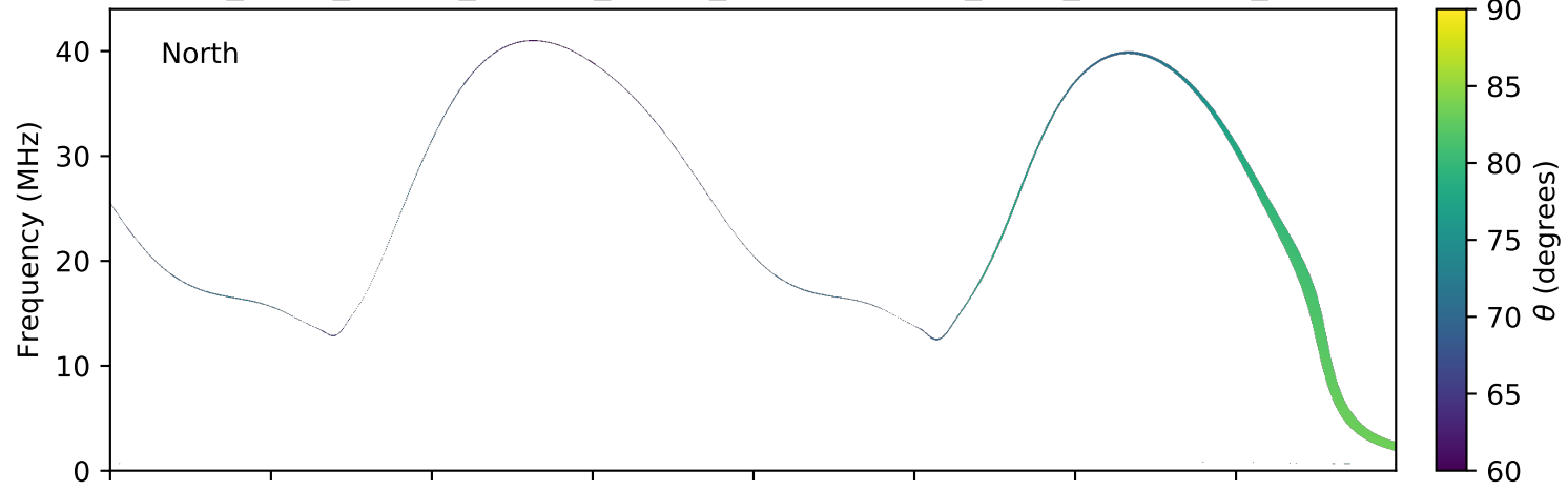
expres_earth_jupiter_europa_jrm09_lossc-wid1deg_3kev_20080707_v01.cdf
