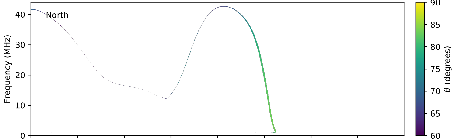
expres_earth_jupiter_io_jrm09_lossc-wid1deg_3kev_20080629_v01.cdf
