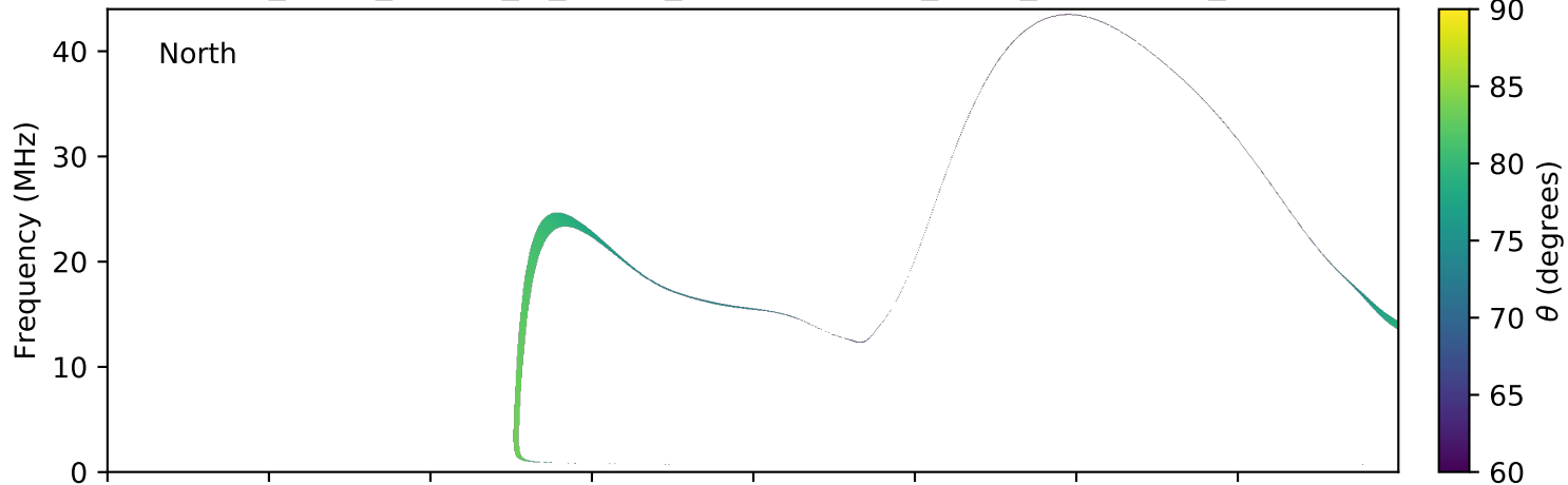
expres_earth_jupiter_io_jrm09_lossc-wid1deg_3kev_20080625_v01.cdf
