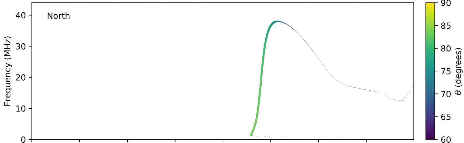
expres_earth_jupiter_io_jrm09_lossc-wid1deg_3kev_20080623_v01.cdf
