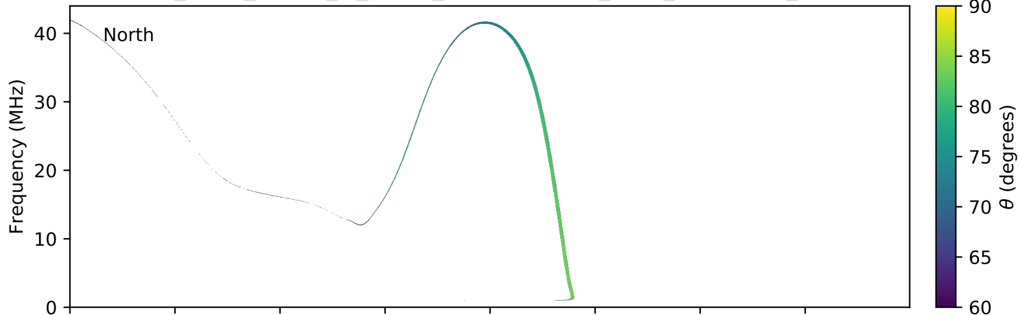
expres_earth_jupiter_io_jrm09_lossc-wid1deg_3kev_20080622_v01.cdf
