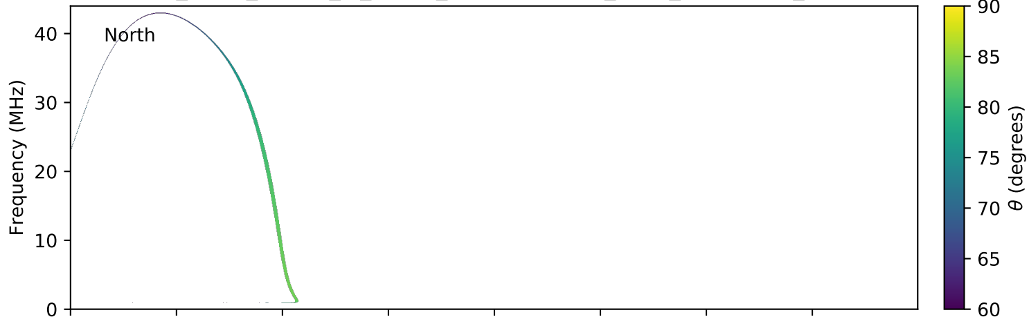
expres_earth_jupiter_io_jrm09_lossc-wid1deg_3kev_20080617_v01.cdf
