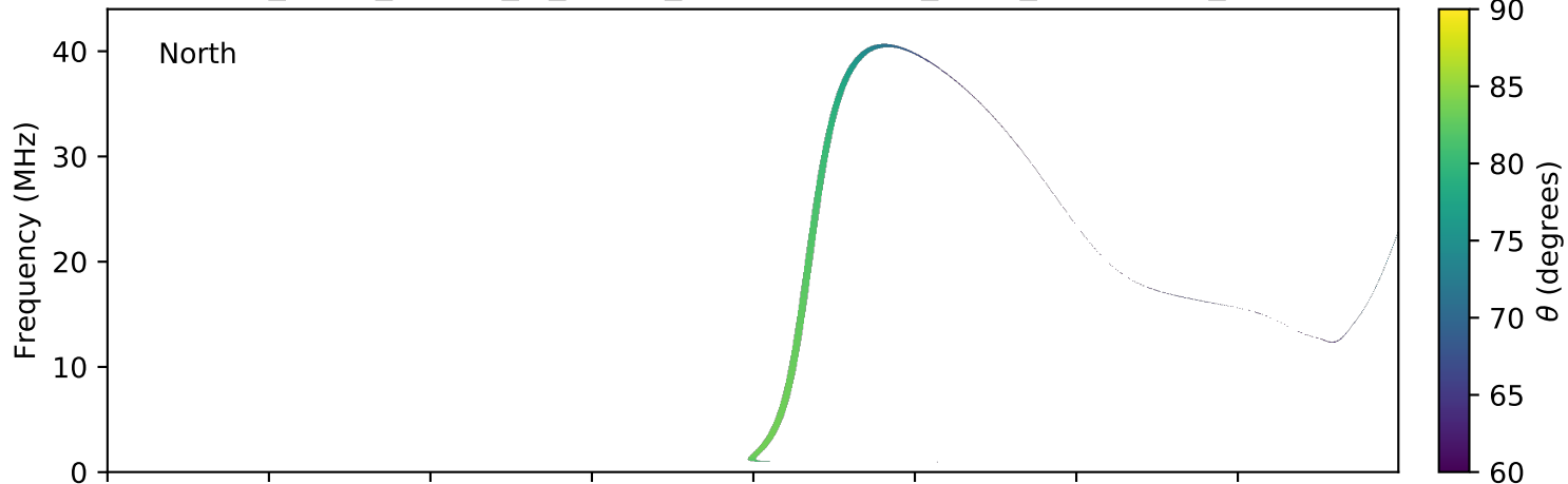
expres_earth_jupiter_io_jrm09_lossc-wid1deg_3kev_20080616_v01.cdf
