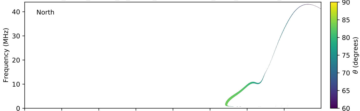
expres_earth_jupiter_io_jrm09_lossc-wid1deg_3kev_20080614_v01.cdf
