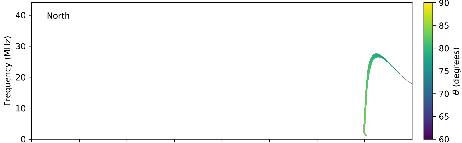
expres_earth_jupiter_io_jrm09_lossc-wid1deg_3kev_20080605_v01.cdf
