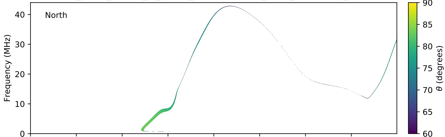
expres_earth_jupiter_io_jrm09_lossc-wid1deg_3kev_20080602_v01.cdf
