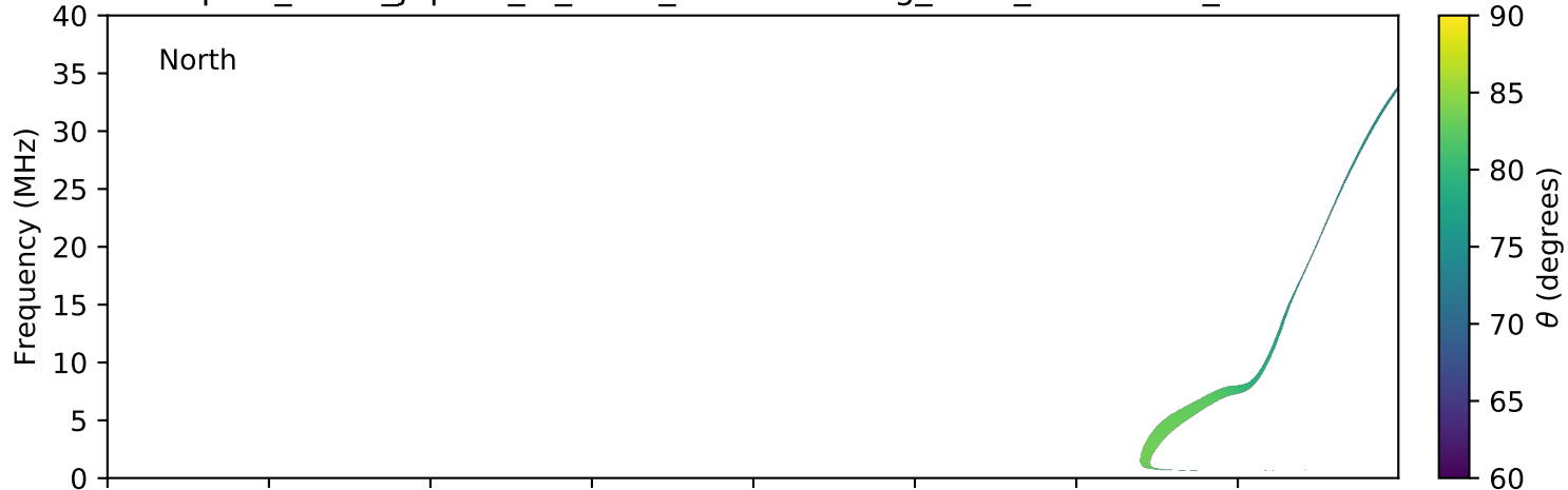
expres_earth_jupiter_io_isaac_lossc-wid1deg_3kev_20080628_v01.cdf
