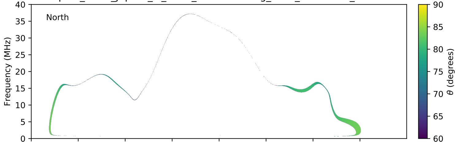
expres_earth_jupiter_io_isaac_lossc-wid1deg_3kev_20080627_v01.cdf
