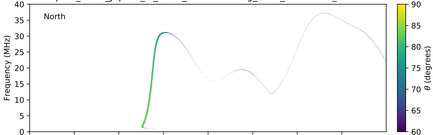
expres_earth_jupiter_io_isaac_lossc-wid1deg_3kev_20080625_v01.cdf
