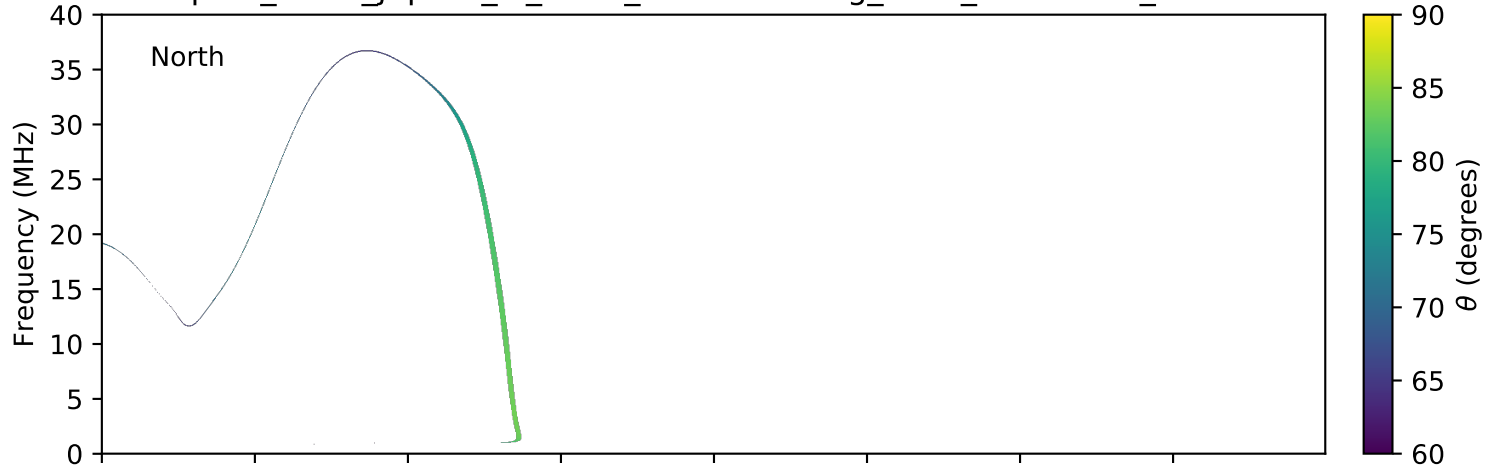
expres_earth_jupiter_io_isaac_lossc-wid1deg_3kev_20080624_v01.cdf
